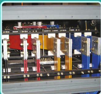
BUS DUCTS
